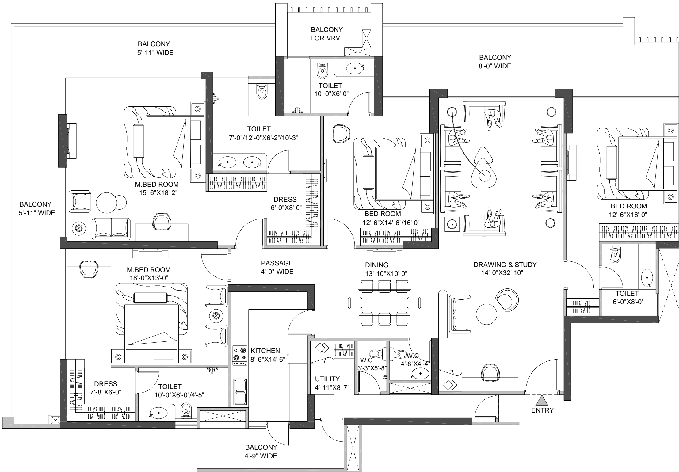
UNIT KEY PLAN
